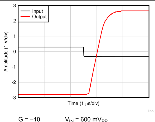
Figure 6-42. Overload Recovery
