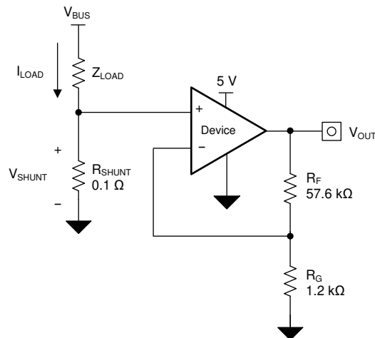
Figure 8-1. OPAx310 in a Low-Side, Current-Sensing Application
