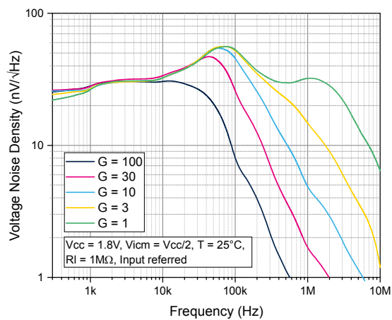
Figure 42. Voltage noise density vs. frequency at V_{CC} = 1.8\text{ V}
