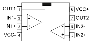
MiniSO8 and SO8 (TSZ152)
