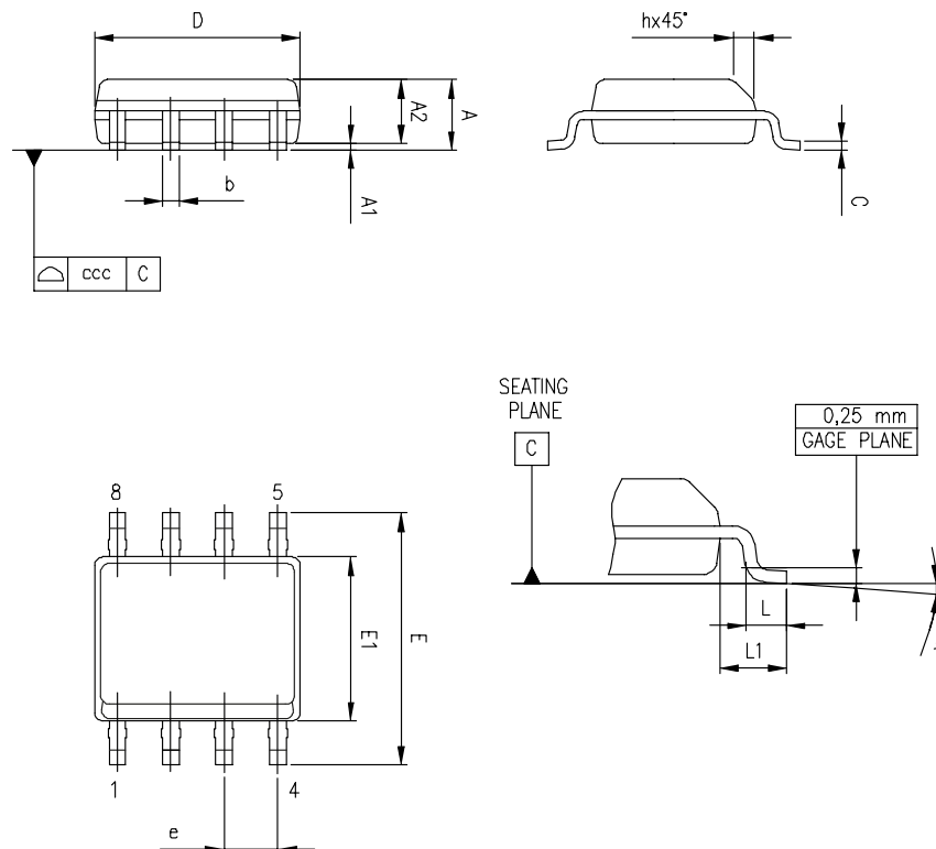
Figure 65. SO8 package outline
