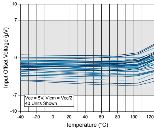
Figure 12. Input offset voltage vs. temperature
