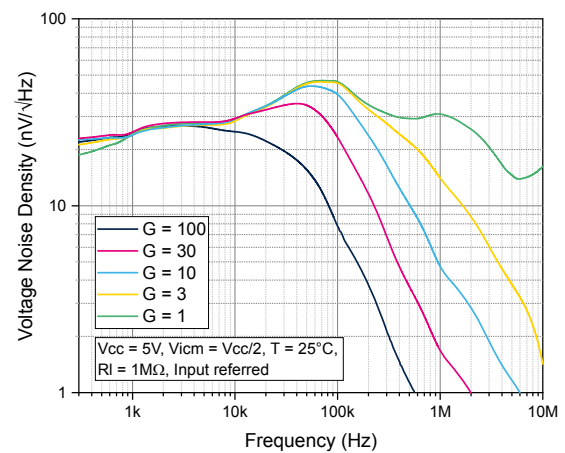
Figure 43. Voltage noise density vs. frequency at V_{CC} = 5\text{ V}
