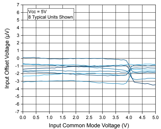
Figure 15. Input offset voltage vs. input common-mode voltage at V_{CC} = 5\text{ V}
