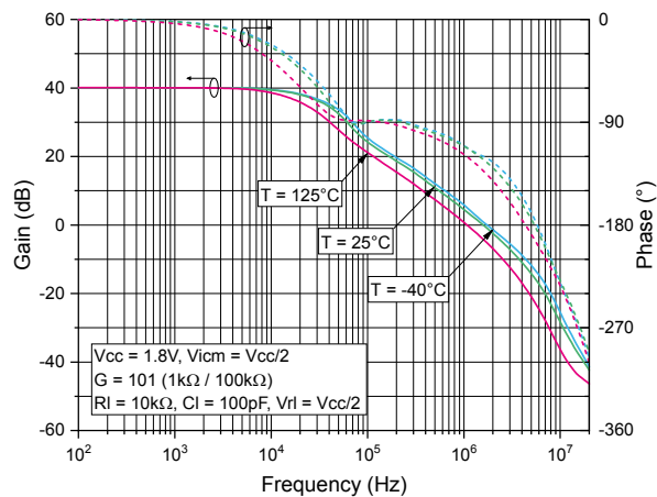
Figure 26. Bode diagram vs. temperature at V_{CC} = 1.8\text{ V}
