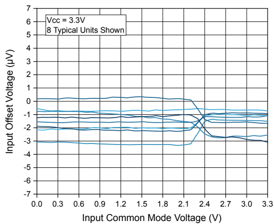
Figure 14. Input offset voltage vs. input common-mode voltage at V_{CC} = 3.3\text{ V}
