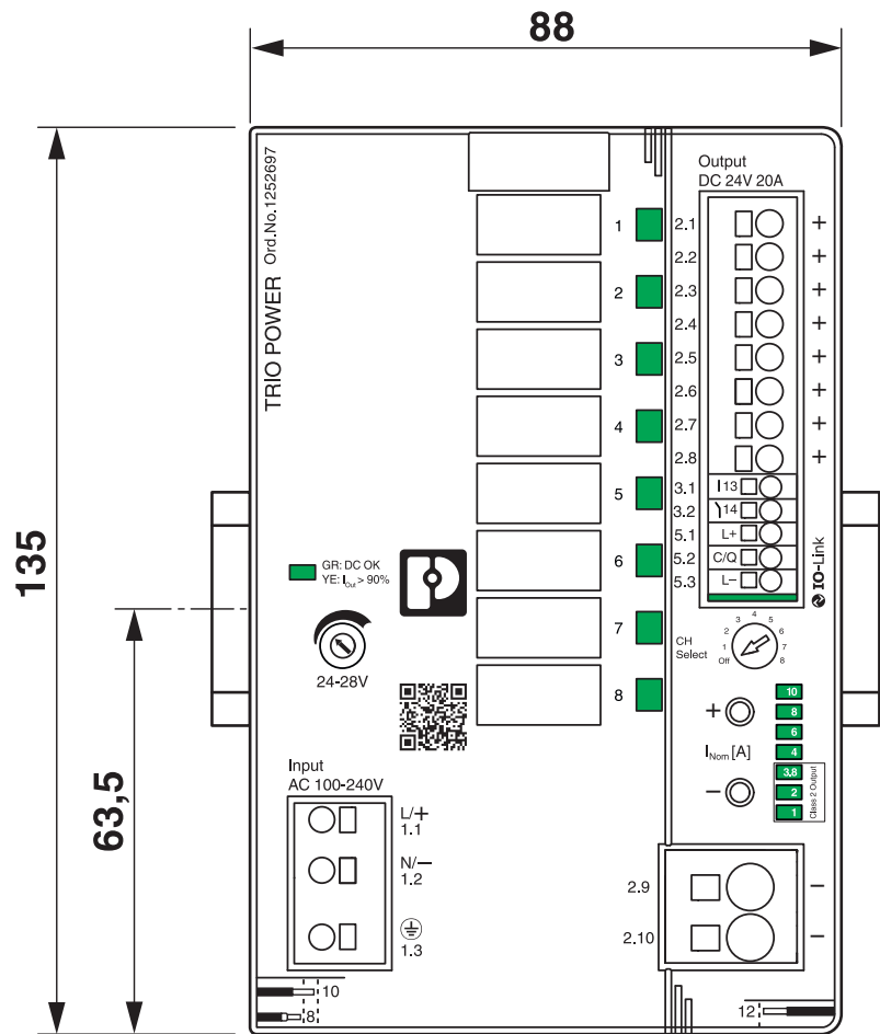
Dimensional drawing
