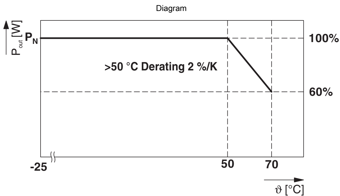
Temperature-dependent derating
