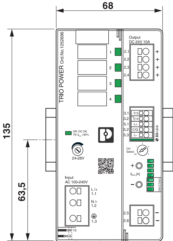
Dimensional drawing
