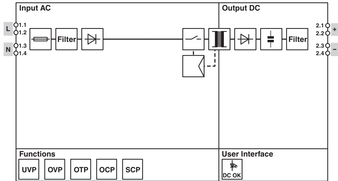
Block diagram
