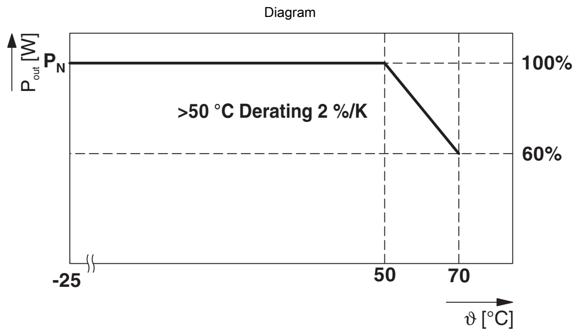
Temperature-dependent derating
