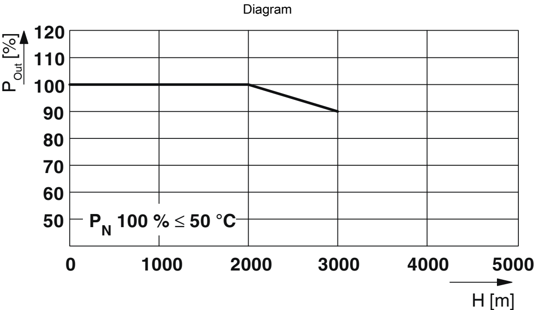
Altitude-dependent derating
