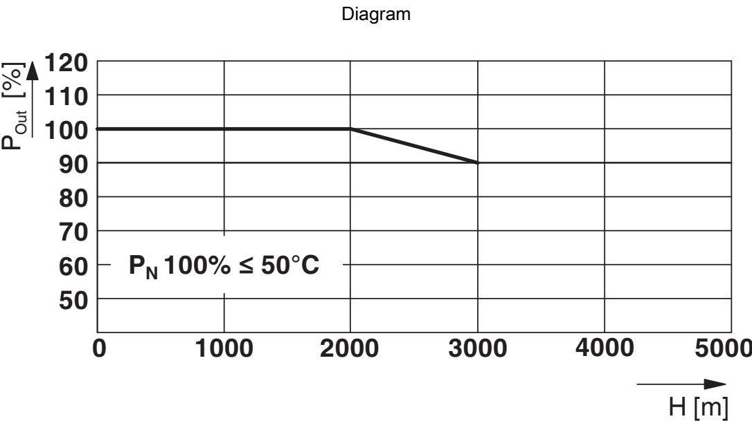
Output power/installation altitude
