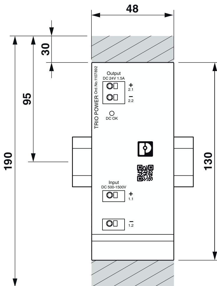
Dimensional drawing
