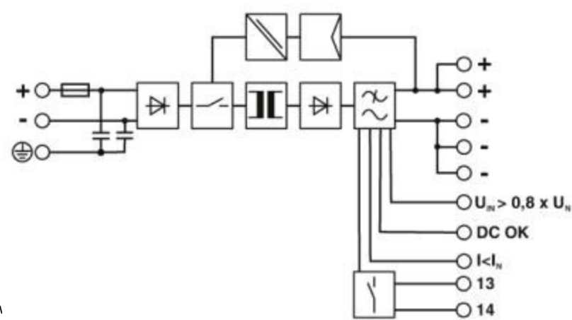
QUINT-PS DC to DC Converter Industrial Power Supply Block Diagram
