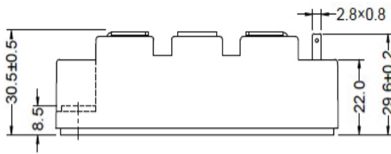
Dimensions-Package S
