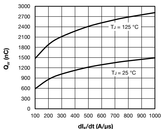
Fig. 16 - Typical Antiparallel Diode Reverse Recovery Charge vs. di_F/dt , V_{rr} = 200\text{ V} , I_F = 50\text{ A}
