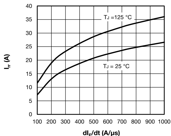
Fig. 15 - Typical Antiparallel Reverse Recovery Current vs. di_F/dt V_{rr} = 200\text{ V} , I_F = 50\text{ A}
