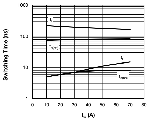
Fig. 8 - Typical Trench IGBT Switching Time vs. I_C T_J = 125\text{ °C} , V_{CC} = 600\text{ V} , R_g = 4.7\text{ }\Omega , V_{GE} = +15\text{ V}/-15\text{ V} , L = 500\text{ }\mu\text{H}
