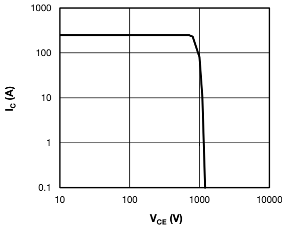
Fig. 17 - Trench IGBT Reverse BIAS SOA T_J = 150^\circ\text{C} , I_C = 250\text{ A} , R_g = 4.7\ \Omega , V_{GE} = +15\text{ V/0 V} , V_{CC} = 700\text{ V} , V_p = 1200\text{ V}
