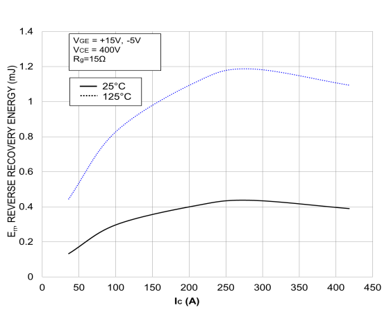
Figure 30. Typical Reverse Recovery Energy vs. I_C
