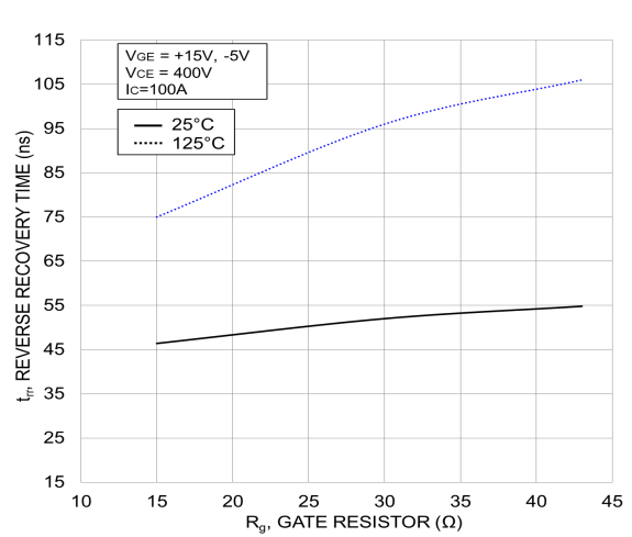
Figure 33. Typical Reverse Recovery Time vs. R_G
