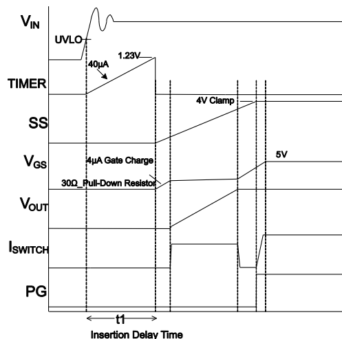
Figure 4: Start-Up Sequence
