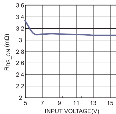
R DS_ON vs. Input Voltage I OUT =1A
