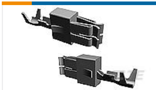
TE Part #927829-2 SPT REC 6.3 Contact SRC Sn
