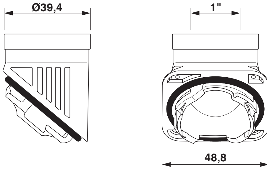
Dimensional drawing
