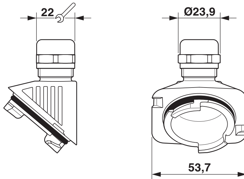
Dimensional drawing
