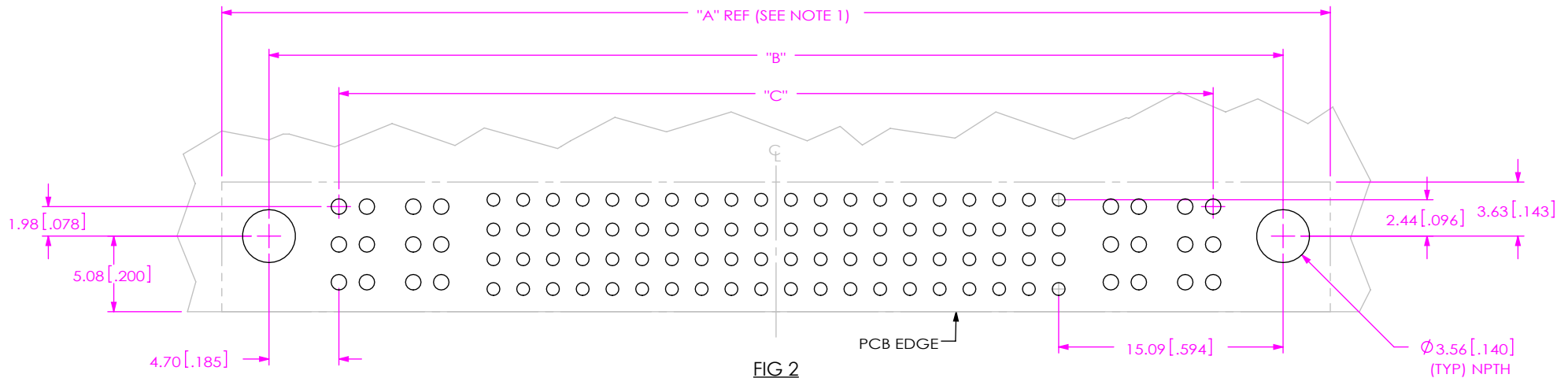
FIG 2 PCB LAYOUT FOR MPSC-XX-XX-XX-01-XX-X-RA-SD SHOWN (SAME AS FIG 1 EXCEPT AS SHOWN)
