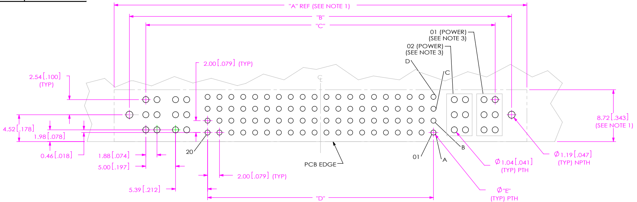
FIG 1 PCB LAYOUT FOR MPSC-XX-XX-XX-01-XX-X-RA-LC SHOWN
