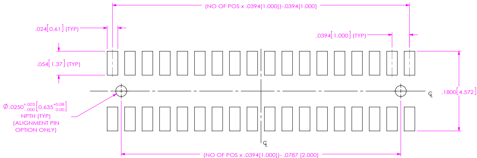
FIG 1 CLM-118-02-XX-D-A FOOTPRINT SHOWN
