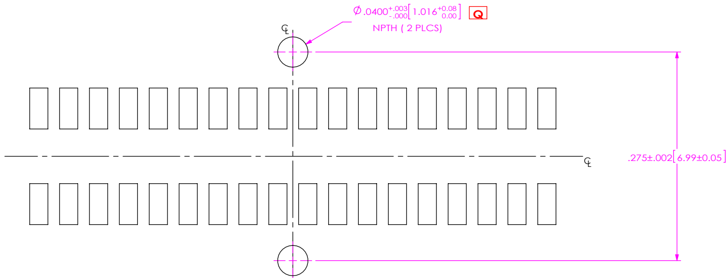
FIG 2 CLM-118-02-XX-D-PA FOOTPRINT SHOWN (SAME AS FIG 1, EXCEPT AS SHOWN)
