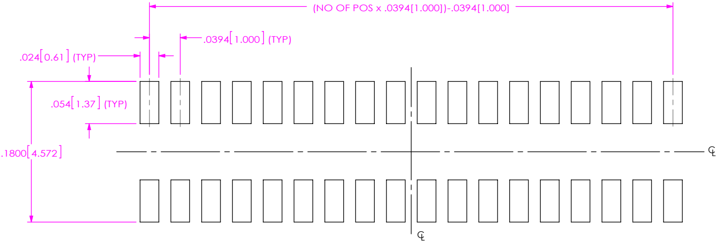
FIG 5 CLM-118-02-XX-D-XX STENCIL SHOWN (SAME AS FIG 1, EXCEPT AS SHOWN)
