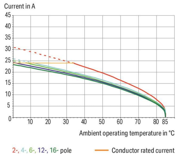
Derating Curve THT female header (232-832) with 1-conductor male connector (731-602) Pin spacing: 7.5 mm / Conductor cross-section: 2.5 mm 2 "f-st" Based on: EN 60512-5-2 / Reduction factor: 0.8
