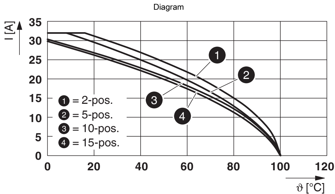
Derating curve for spring-cage terminals ST 4/1P.. and ST 4/2P.. with all plug versions SP 4/... The derating curves are determined by multiplying the values of the base curves by the factor 0.8.
