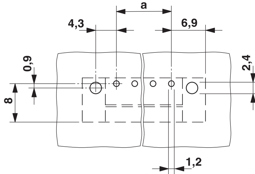
Dimensional drawing
