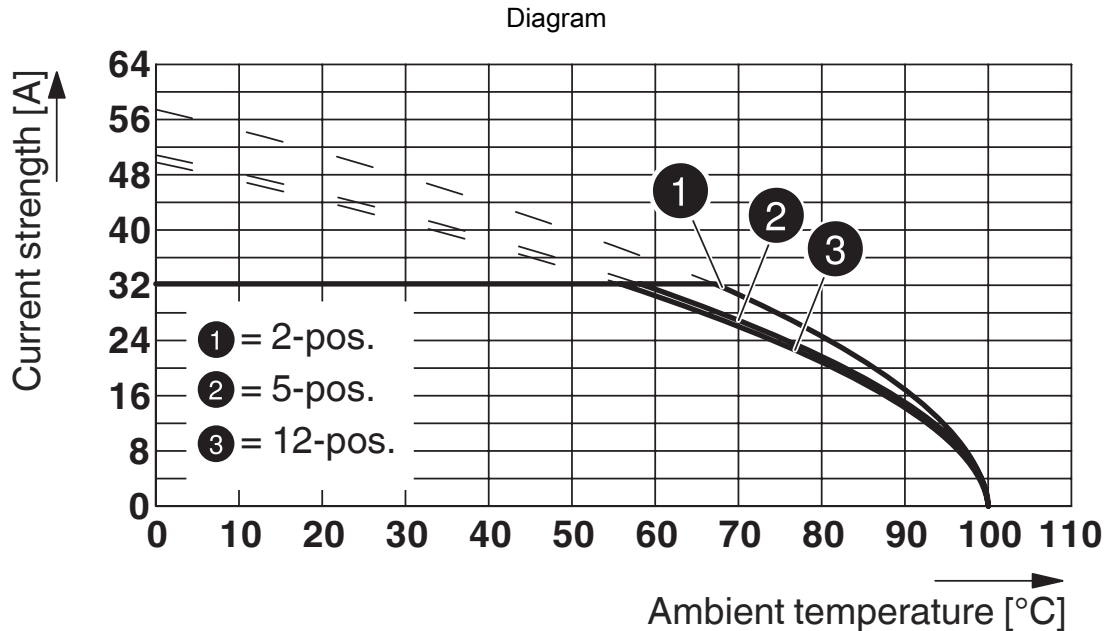
Type: PC 5/...-ST1-7,62 with PC 5/...-GU-7,62 P26 THT R.. Conductor cross section: 6 mm 2
