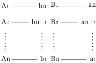
Cable connection
