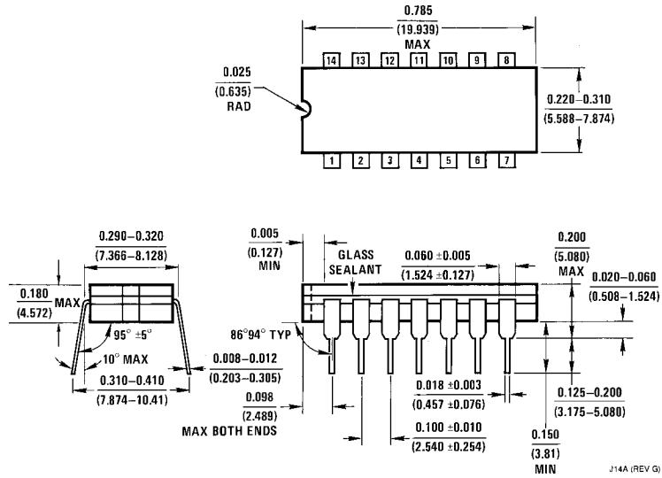
14-Lead Ceramic Dual-In-Line Package (J) Order Number 54LS05DMQB or DM54LS05J NS Package Number J14A
