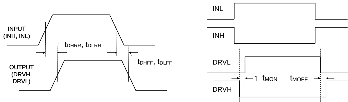
Figure 1: Timing Diagram
