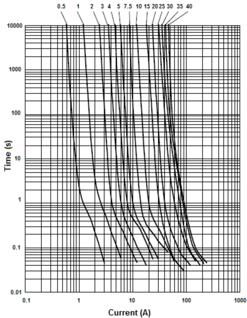
Time Current Curve Graph
