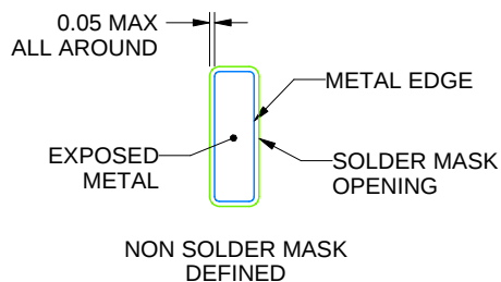
SOLDER MASK DETAIL
