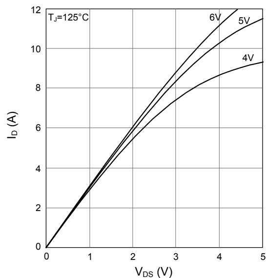
Figure 5. Typ I_{D\_LS} vs. V_{DS} at T_J=125^\circ\text{C}
