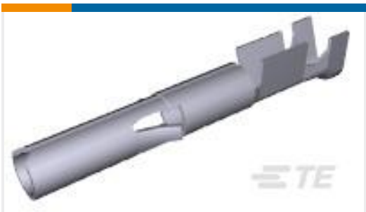
TE Part # 350689-7 UMNL SOK 24-18 AUBR L/P
