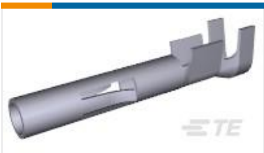
TE Part # 350550-7 UMNL SOK 20-14 AU/BR L/P
