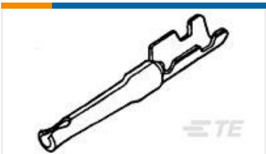
TE Part # 1658686-1 SOCKET CONTACT,22 DF,STRIP,22-
