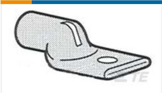
TE Part # 325905 TERMINAL,AMPOWER 350MCM 1/2
