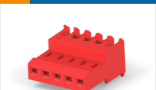
TE Part #3-641239-6 Nylon Gold Plated Receptacle: 2.54 mm, no Mating Alignment
