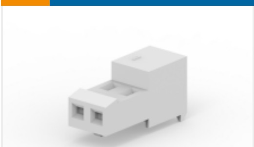
TE Part #3-640440-3 MTA Receptacle: Nylon, Tin Plated, 2.54 mm
