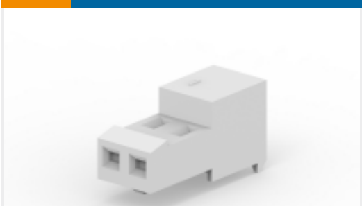
TE Part #3-640442-9 MTA Receptacle: Nylon, Tin Plated, 2.54 mm
