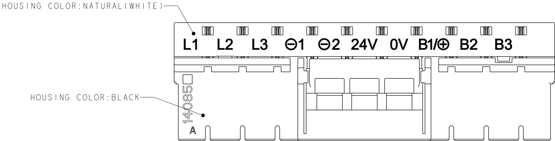
1-2289080-2 (11 POSITION KEYING: X)
