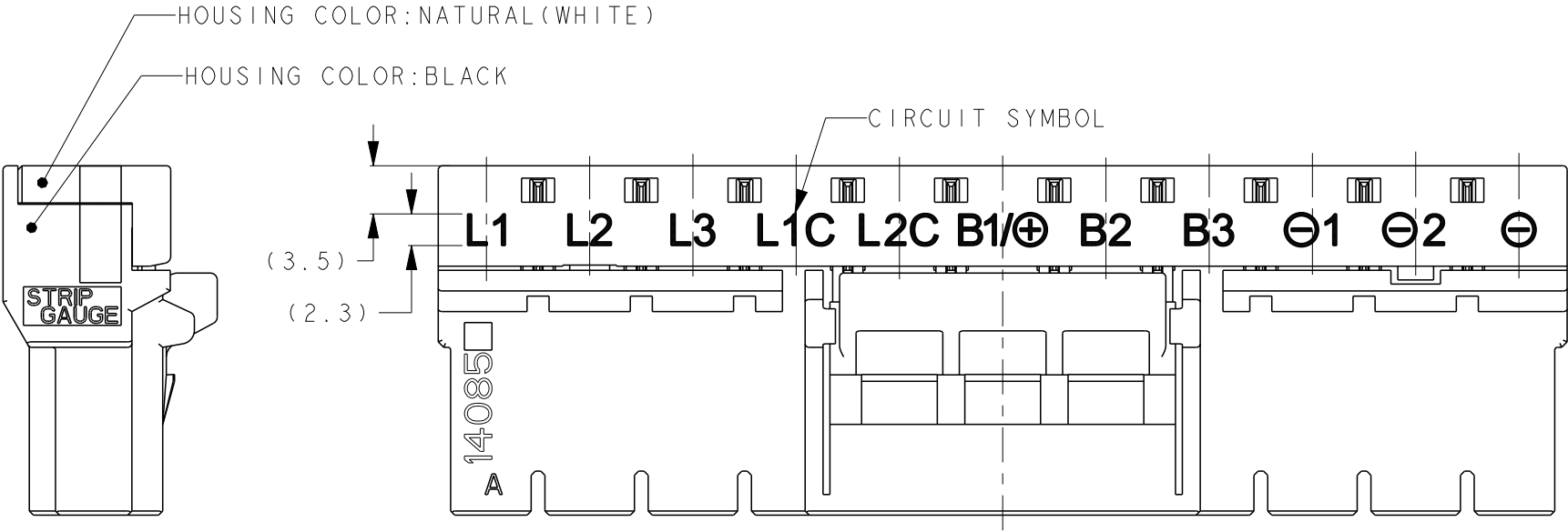
1-2289080-2 (11 POSITION KEYING: X)
