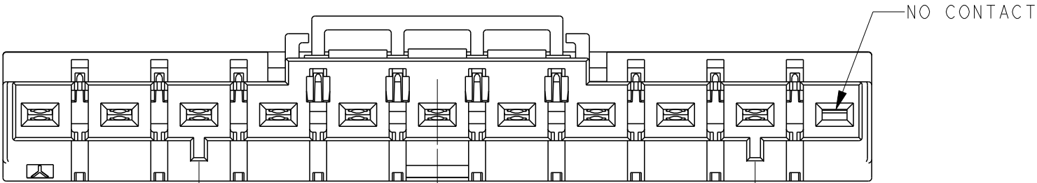
1-2289080-3 (10 POSITION KEYING: Y)
