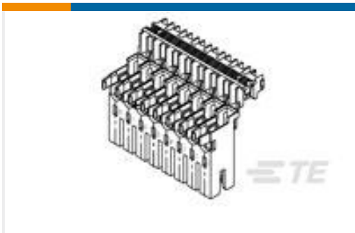
TE Part #1-282045-2 AMP MONO-SHAPE P.C.B.CONN5P. G
