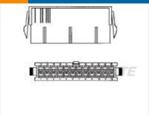
TE Part # 1586018-6 6P PM PLUG VAL-U-LOK V0
