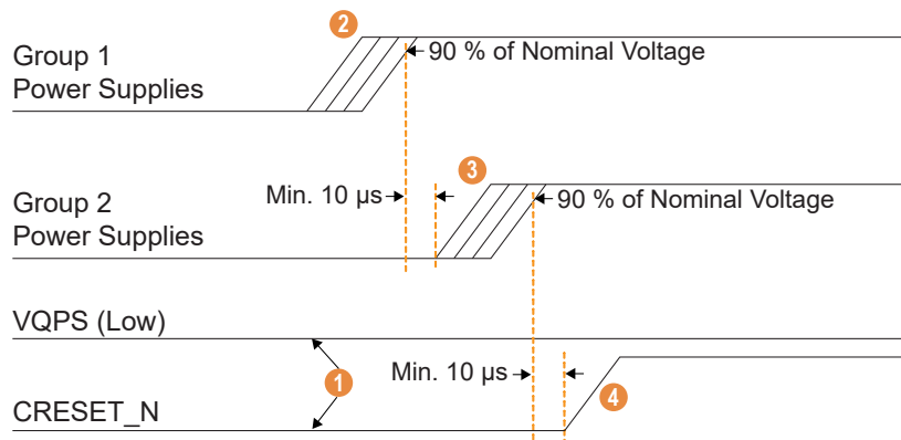
Figure 46: Power-Up Sequence
