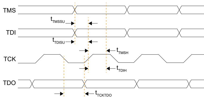
Figure 51: JTAG Timing Waveform
