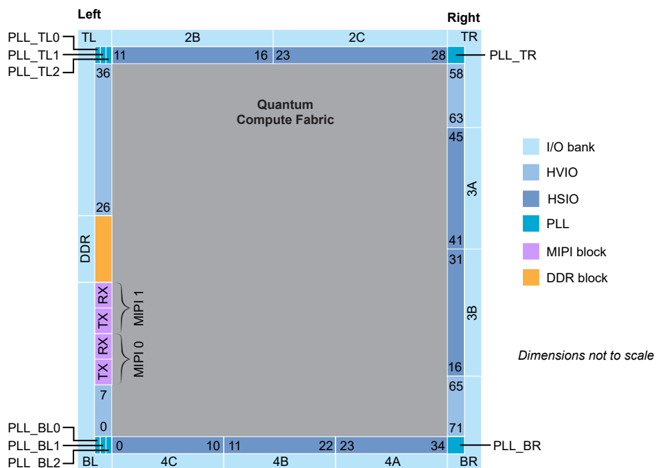
Figure 52: Floorplan Diagram for J361 and M361 Packages
