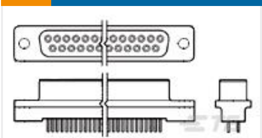
TE Part # 5745076-3 HD-20 RCPT 9P VERT FFSCRLK
