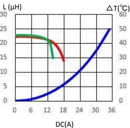
5. CDPQ2419NP-220LB-AL343
