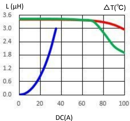
1. CDPQ2419NP-3R3LB-AL51
