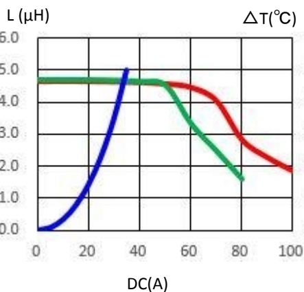
2. CDPQ2419NP-4R7LB-AL73
