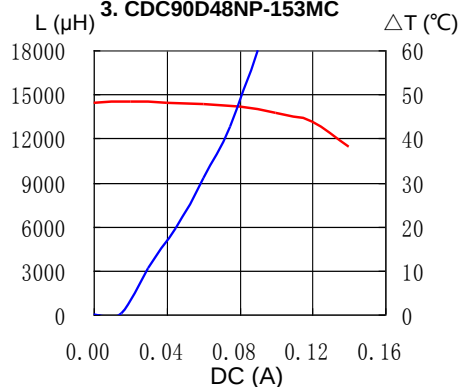
3. CDC90D48NP-153MC
