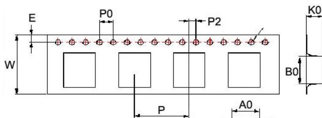
Tape Dimensions
