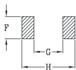
Suggested PWB Layout
