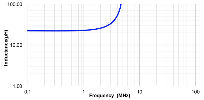
VSHB1054T-220MC
