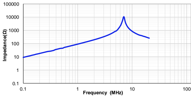
VSHB1054T-150MC
