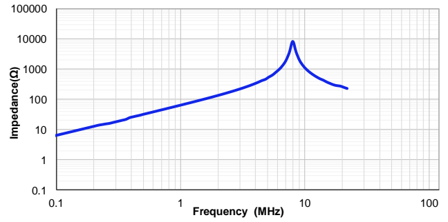
VSHB1054T-100MC
