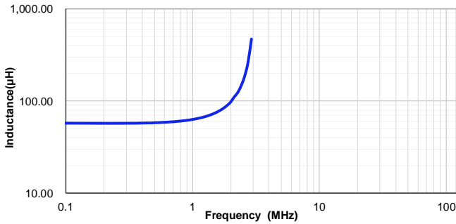
VSHB1054T-560MC
