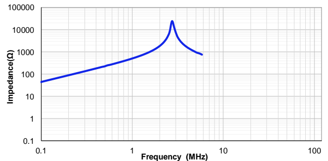
VSHB1054T-680MC
