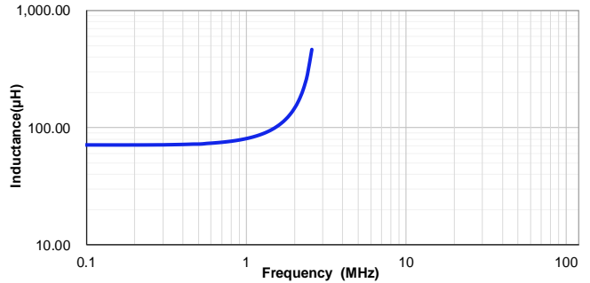
VSHB1054T-680MC
