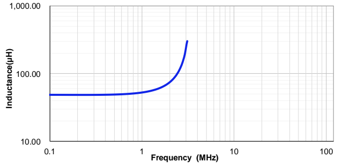
VSHB1054T-470MC
