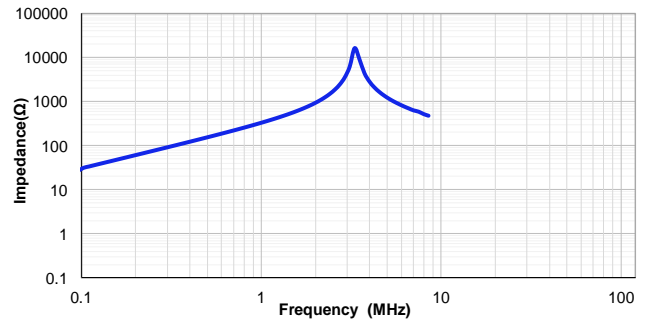
VSHB1054T-470MC
