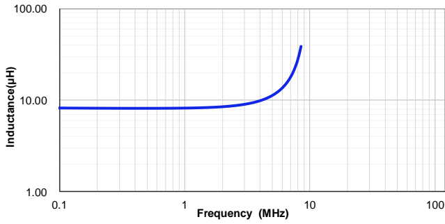
VSHB1054T-8R2MC
