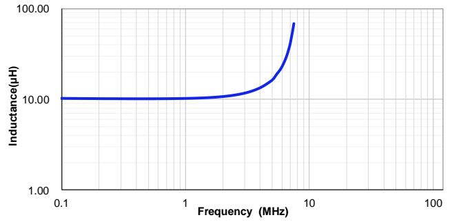
VSHB1054T-100MC
