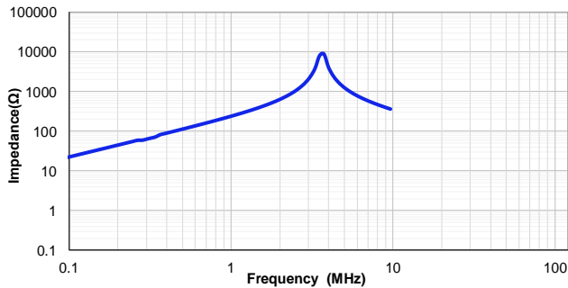
VSHB1054T-330MC
