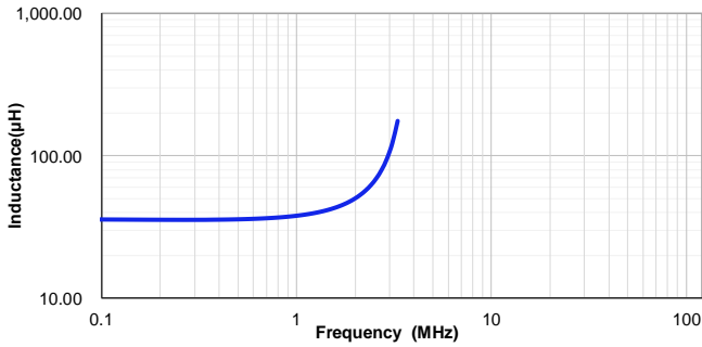
VSHB1054T-330MC
