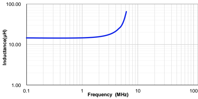
VSHB1054T-150MC
