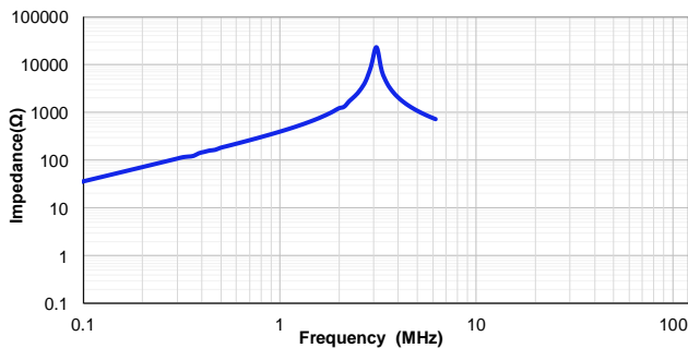
VSHB1054T-560MC
