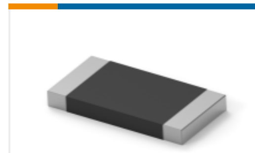
TE Part #5-2176422-5 TLRP 2512 3.0W R012 1% 50PPM 4K RL
