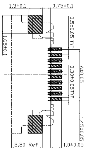
Sold Pad Pattern
