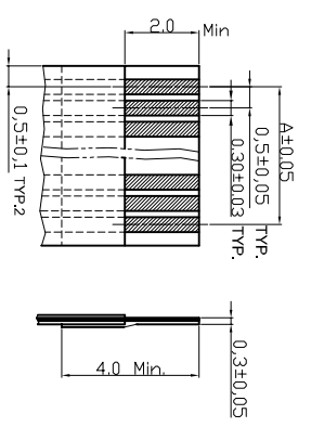
Accommodated FFC/FPC
