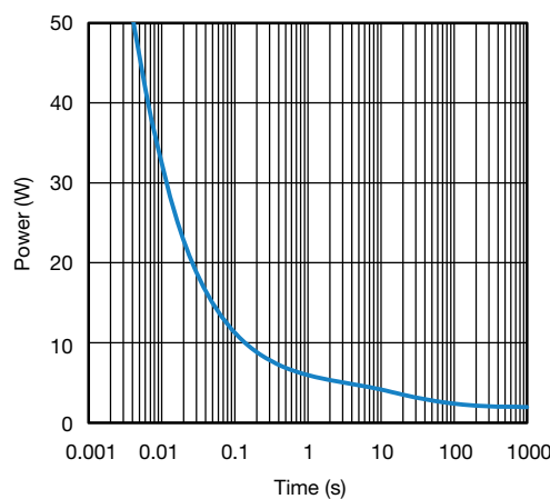
Single Pulse Power, Junction-to-Ambient
